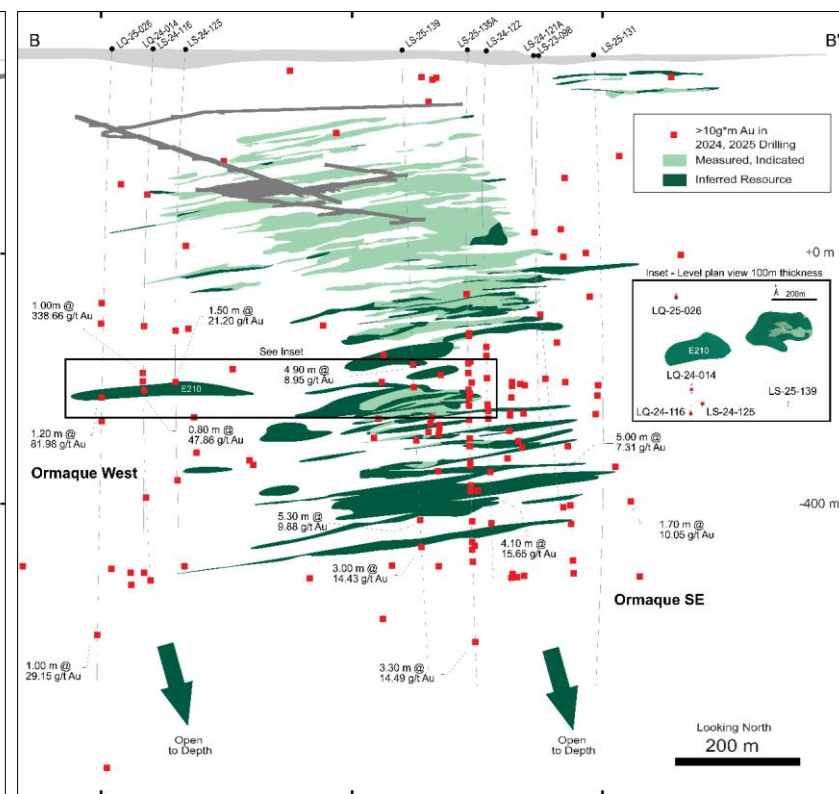
Long section through the Ormaque deposit showing >10 g*m intercepts outside the Ormaque resource and highlighted drillhole intercepts. Flat-lying vein intercepts extend 200 to 300 metres west beyond the Ormaque resource.
