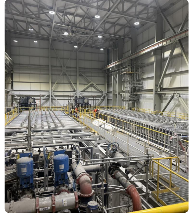
Tailings filtration
