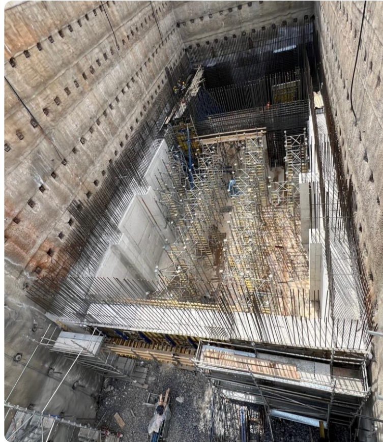
Primary Crusher – wall progress
