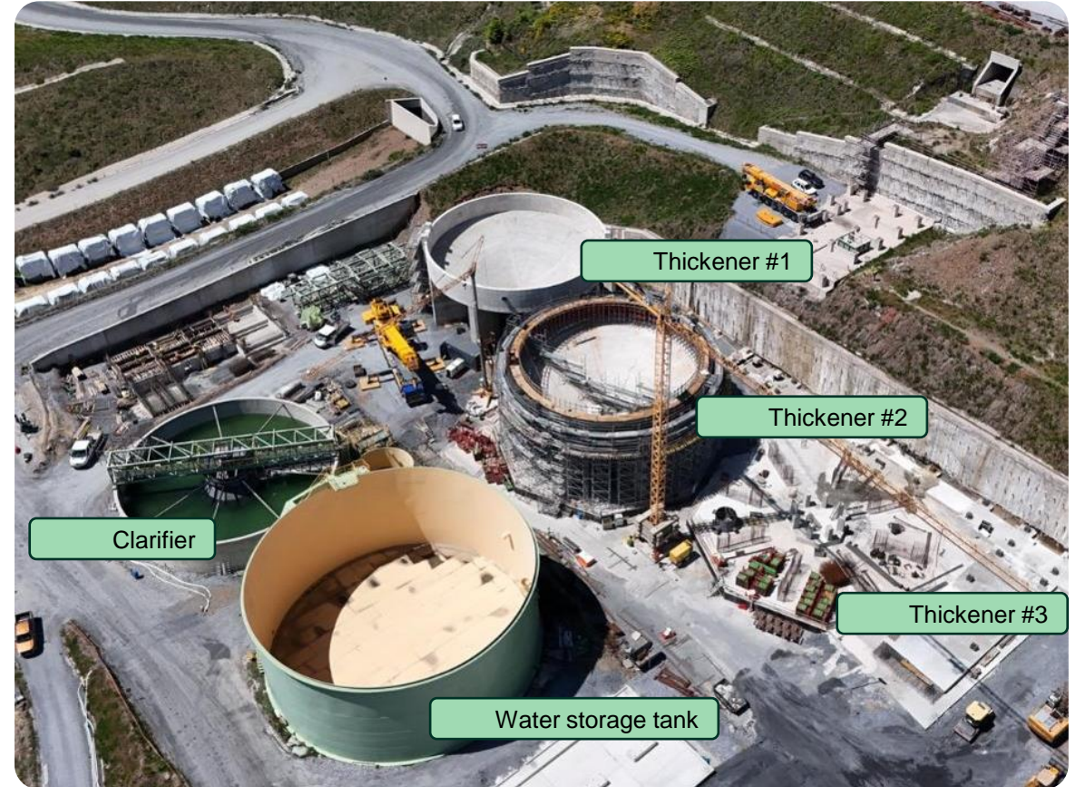
Thickeners – concrete works complete on first, progressing on two, and construction on third thickener has commenced, with the base completed.
